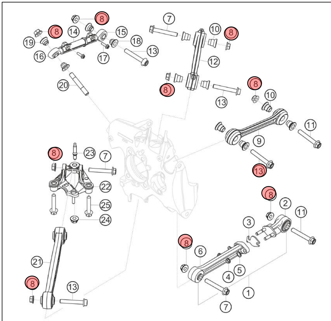
The highlighted connections 8 and 13 shown above require 120 Nm torque.
